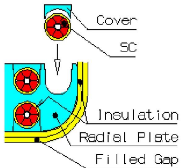
Fig. 2: The conductor is insulated with glass/Kapton tapes and is placed inside the groove of the radial plate
