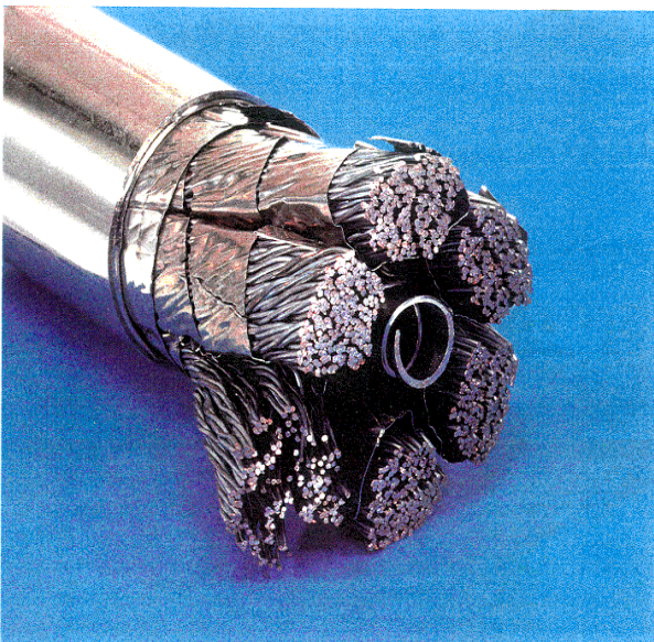
Fig.1: TFMC conductor: 720 Nb 3 Sn and 360 Cu strands cabled around a centre spiral and inserted in a 316LN jacket
